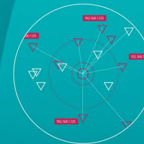
BOTNET PROTECTION
