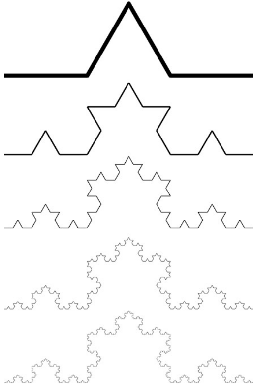
Koch curve
